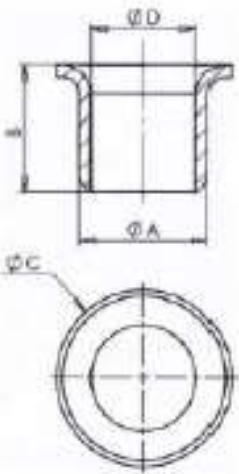
Manufacture of capsules and rim eyelets
